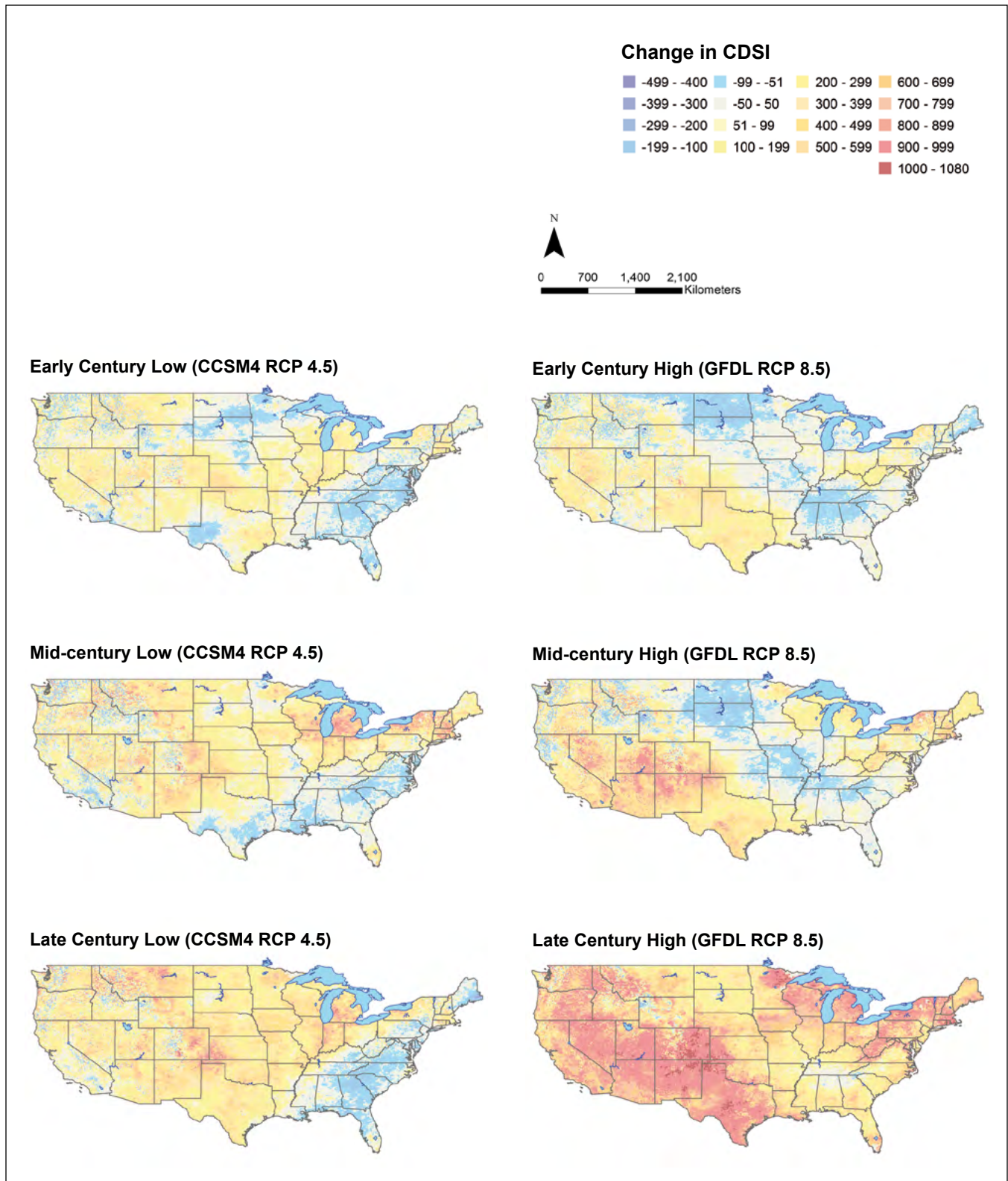
Figure 9.—Mapped projections of changes in CDSI for conterminous United States by 30-year time period and climate scenario. Each future 30-year interval is generally expected to experience more drought events (increased index score), according to the two scenarios used in this study. However, most regions could see more frequent or more intense droughts by end of century, regardless of scenario. More than 45 percent of the area in the Midwest, Northeast, Southern Plains, Northwest, and Southwest regions is projected to see an increase of at least 700 CDSI under the high scenario. Time periods: early century (2010–2039); mid-century (2040–2069); late century (2070–2099).
