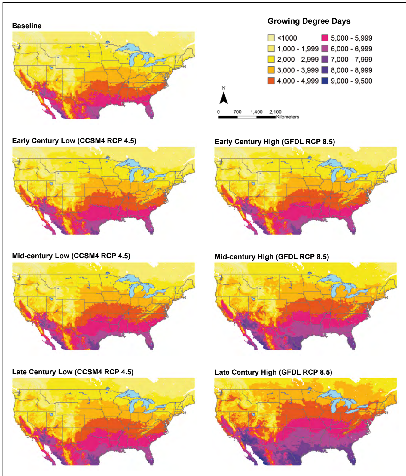
Figure 2.—Maps of baseline and projections of mean growing degree days for conterminous United States by 30-year time period using a low (RCP 4.5; see text for explanation) or high (RCP 8.5; see text for explanation) climate scenario. The maps show an accumulation of growing degree days. Time periods: baseline (1980–2009); early century (2010–2039); mid-century (2040–2069); late century (2070–2099).
