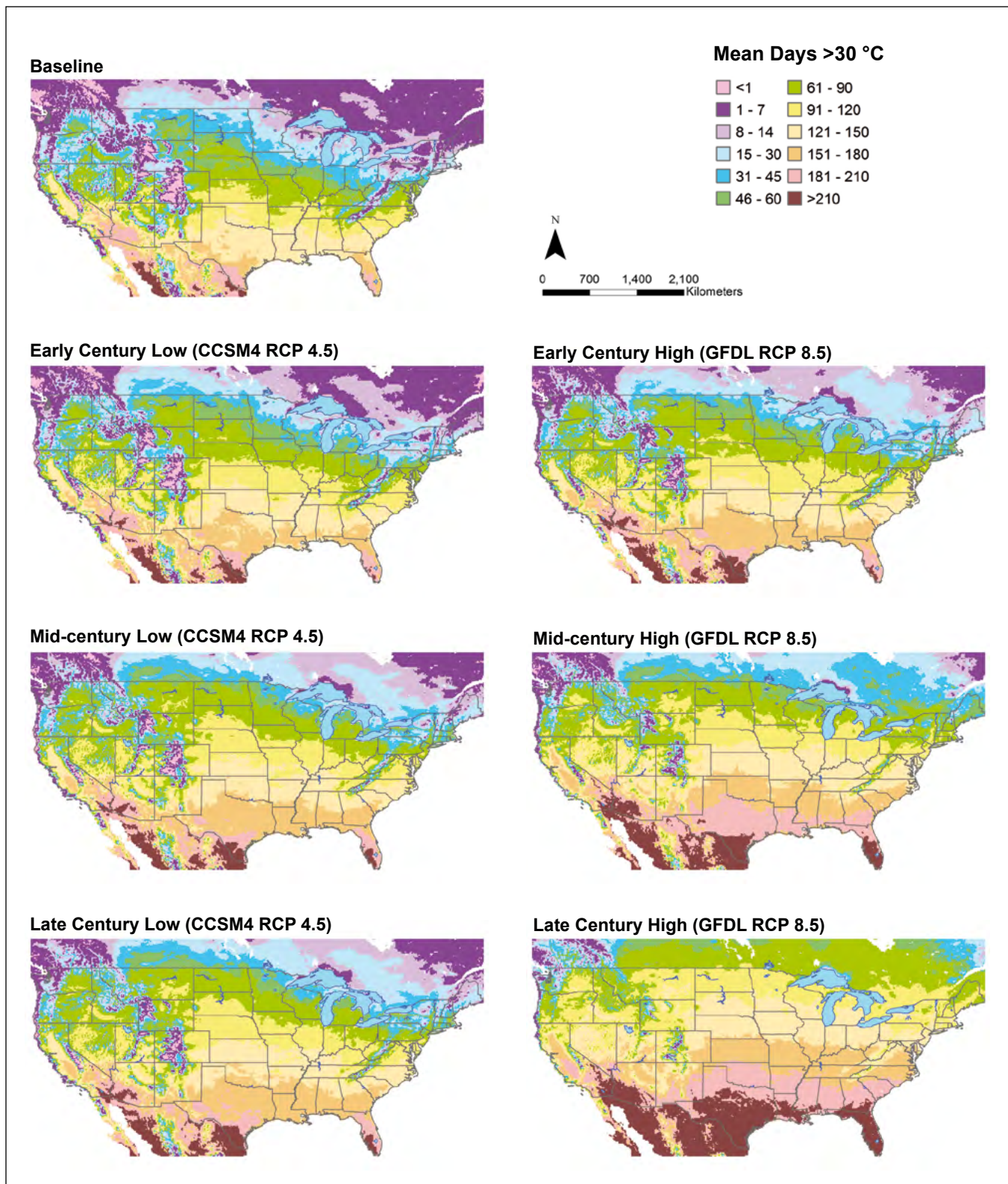
Figure 6.—Maps of baseline and projections of mean number of days per year with temperature above 30 °C (reflecting the heat zone metric) for conterminous United States by 30-year time period using a low (RCP 4.5; see text for explanation) or high (RCP 8.5; see text for explanation) climate scenario. While 30 °C does not represent a species-specific physiological threshold, it is acknowledged that temperatures above this temperature exceed a general optimal threshold for photosynthesis for C_3 plants (Rennenberg et al. 2006). Time periods: baseline (1980–2009); early century (2010–2039); mid-century (2040–2069); late century (2070–2099).
