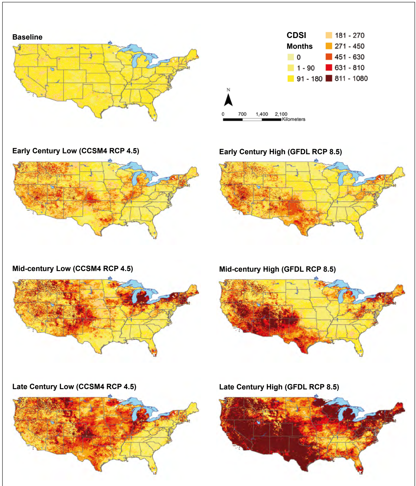
Figure 8.—Maps of baseline and projections of Cumulative Drought Severity Index (CDSI) for conterminous United States by 30-year time period using a low (RCP 4.5; see text for explanation) or high (RCP 8.5; see text for explanation) climate scenario. The yearly CDSI values were accumulated over each of the 30-year periods. The range of CDSI values for the 360 months in a 30-year period can range from 0 (no months with any drought) to 1080 (every month has an extreme drought). Time periods: baseline (1980–2009); early century (2010–2039); mid-century (2040–2069); late century (2070–2099).
