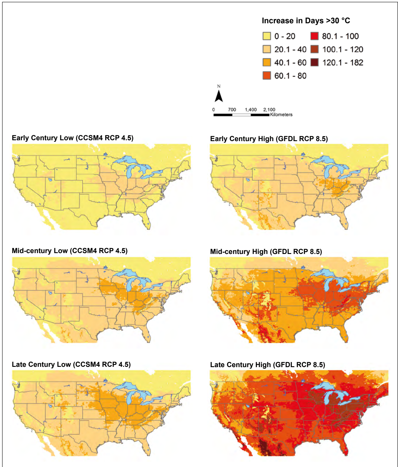
Figure 7.—Mapped projections of changes in number of days per year with temperature above 30 °C for conterminous United States by 30-year time period and climate scenario. Heat zones are projected to expand everywhere, but particularly in the Midwest, parts of the Northeast, and the Rocky Mountains by the end of the century, especially under the high climate scenario. Time periods: early century (2010–2039); mid-century (2040–2069); late century (2070–2099).
