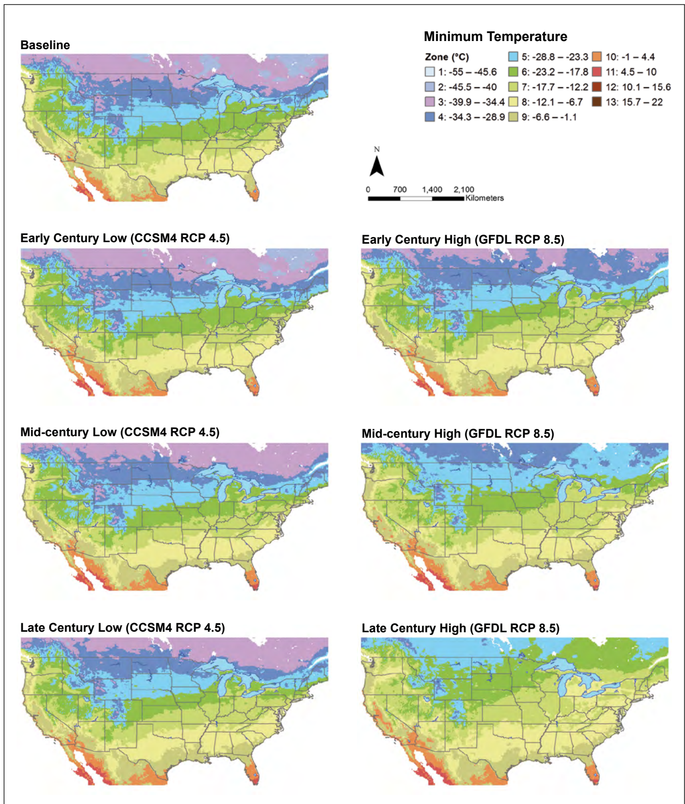
Figure 4.—Maps of baseline and projections of mean absolute minimum temperature (reflecting the plant hardiness zone metric) for conterminous United States by 30-year time period using a low (RCP 4.5; see text for explanation) or high (RCP 8.5; see text for explanation) climate scenario. To define the coldest day per year, daily minimum temperatures were identified within the period July 1 to June 30, with the year assigned to the first 6 months of the 12-month period. Zone categories follow the USDA definitions (Cathey 1990). Time periods: baseline (1980–2009); early century (2010–2039); mid-century (2040–2069); late century (2070–2099).
