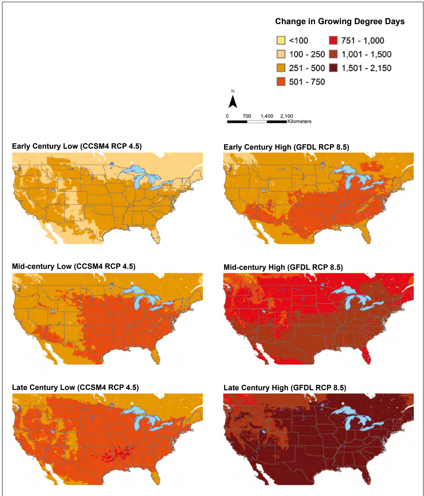
Figure 3.—Mapped projections of increase in growing degree days for conterminous United States by 30-year time period and climate scenario. Projections suggest a ubiquitous increase across the United States, with slightly less change in the Northeast and much greater increases in the Southwest under the high scenario. Time periods: early century (2010–2039); mid-century (2040–2069); late century (2070–2099).
