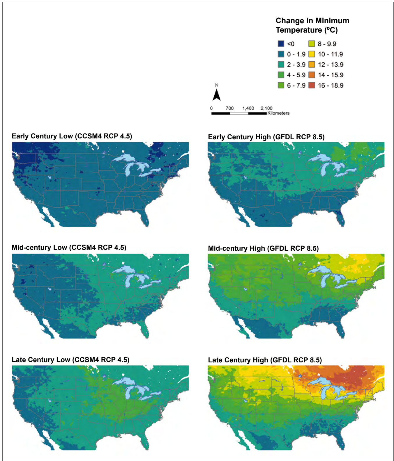
Figure 5.—Mapped projections of changes in minimum temperature for conterminous United States by 30-year time period and climate scenario. Plant hardiness zones are projected to have the greatest changes in the Northeast and Northern Plains. Time periods: early century (2010–2039); mid-century (2040–2069); late century (2070–2099).
